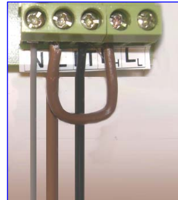
Wiring Photograph: Timer + High Speed
