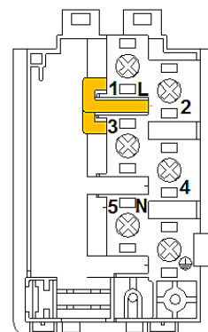
Heater de-rated to 2kW
