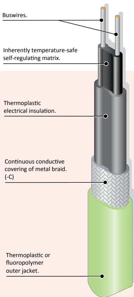
CRJ Self Regulating Cable - Dispensed by the metre
