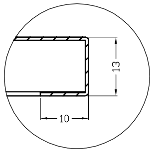
F (1:10)
