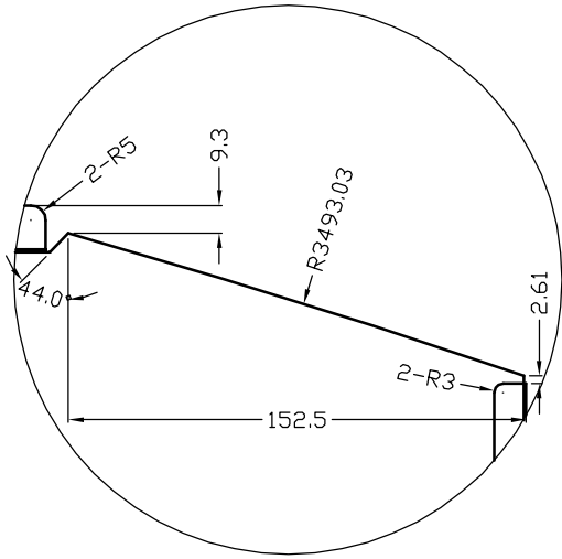
E (1:3)
