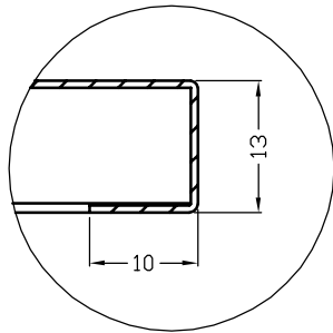
F (1:10)
