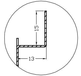
G (1:10)
