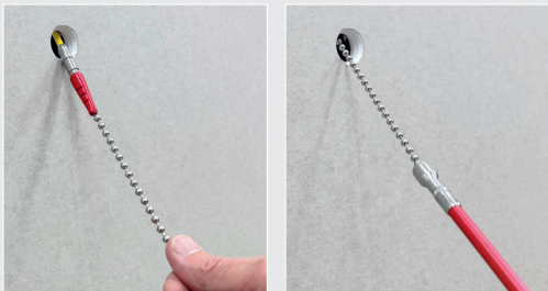
RG7 – Guiding head incl. swivel with front thread and eyelet Ø 7 mm
