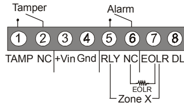
Figure 1: Terminal Block
