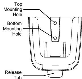
Figure 2: INF-REMCON Mounting Bracket
