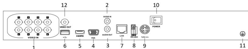
Figure 1. 12 Rear Panel of DS-7200HQHI-F2/N
