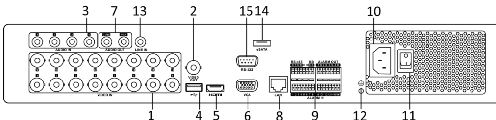
Figure 1. 14 Rear Panel of DS-7300HQHI-F4/N
