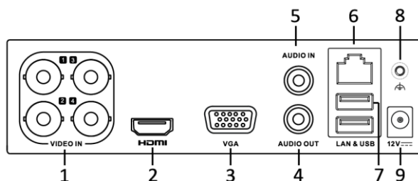
Figure 1. 8 Rear Panel of DS-7100
