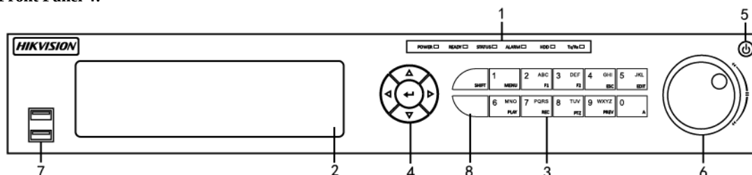
Figure 1. 4 Front Panel of DS-7300HQHI-F/N
