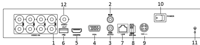
Figure 1. 11 Rear Panel of DS-7200HQHI-F1/N
