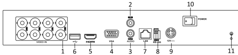
Figure 1. 10 Rear Panel of DS-7200HGHI-E1/E2
