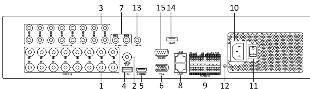
Figure 1. 15 Rear Panel of DS-8100HQHI-F8/N
