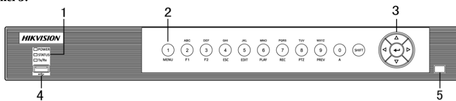
Figure 1. 3 Front Panel of DS-7200HUHI-F/N
