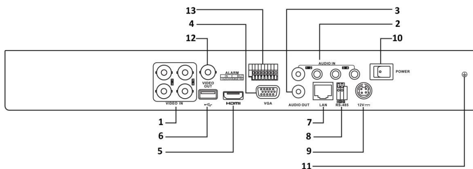
Figure 1. 13 Rear Panel of DS-7200HUHI-F/N
