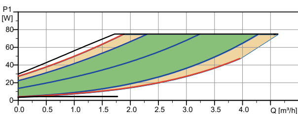
Constant pressure
