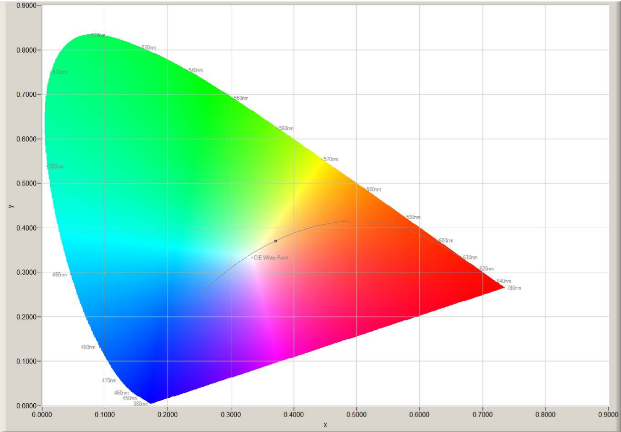
Figure 2: CIE 1931 diagram.
