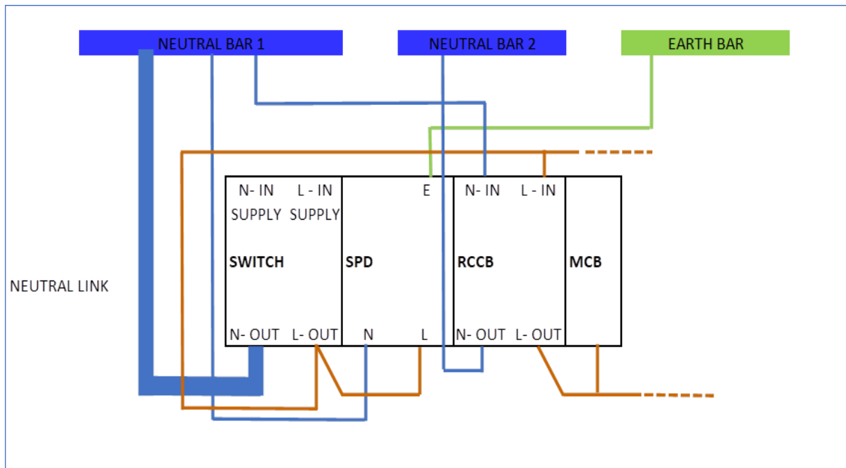
Wiring diagram for H6820s surge device.....
