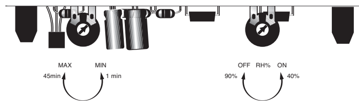
Diagram 5: HUMIDITY OPERATED TIME DELAY CONTROL
