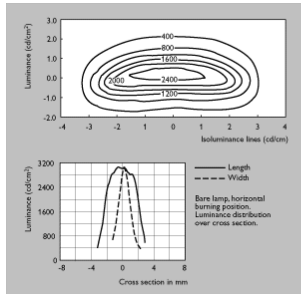
MASTERC CDM-TC 35W
