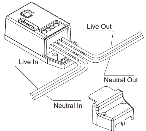
Wiring Instructions
