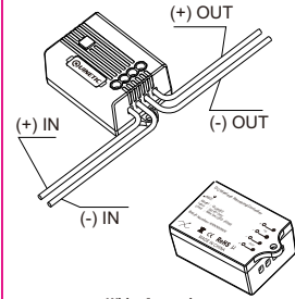
Wiring Instructions
