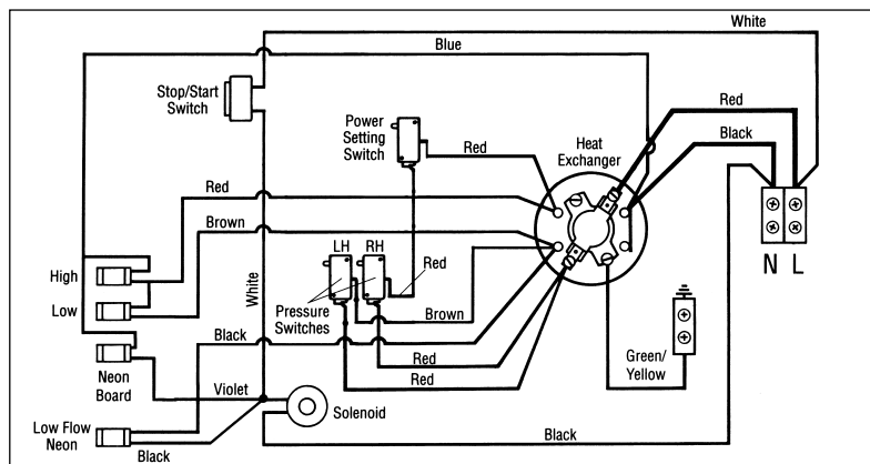
Figure 1.1 Internal Circuit Diagram- Carousel 8.7kW
