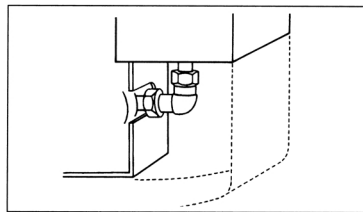
Figure 4.9 Connection of pipe to inlet (top entry shown).
