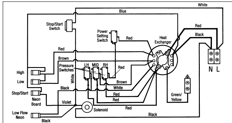
Figure 1.1 Internal Circuit Diagram- Carousel 9.8/10.8kW
