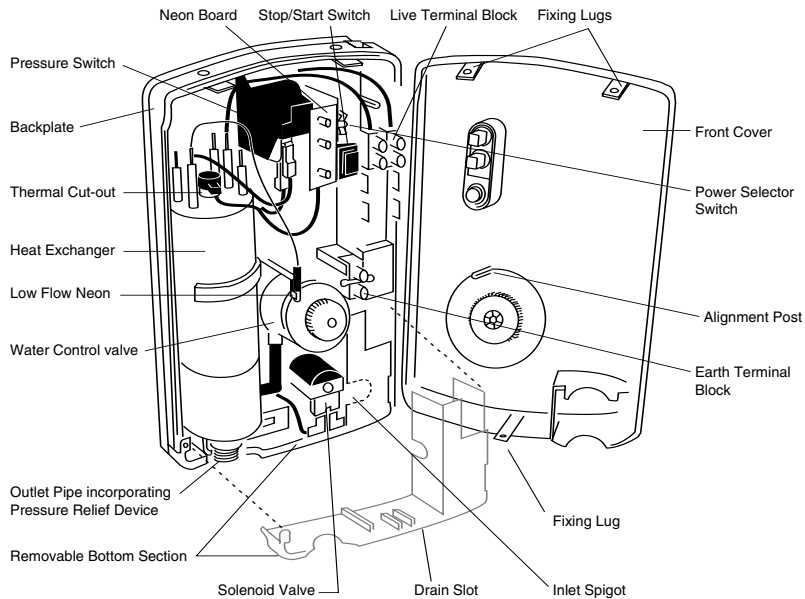
Figure 1.0 Major Internal Components
