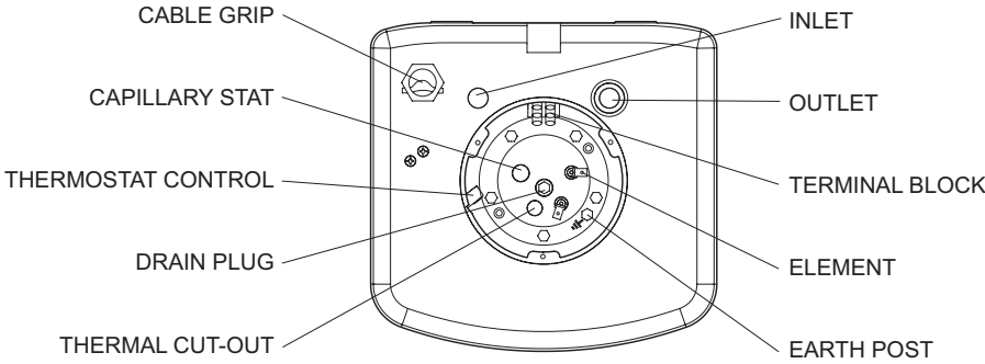
Fig.1 - Internal Layout.
