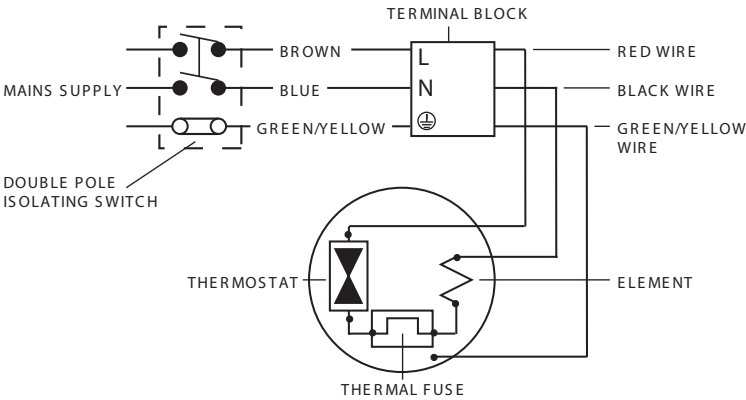
Fig.2 Wiring Diagram.
