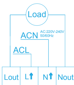
Fig.3 Wiring Diagram
