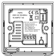
Fig. 2 Back View
