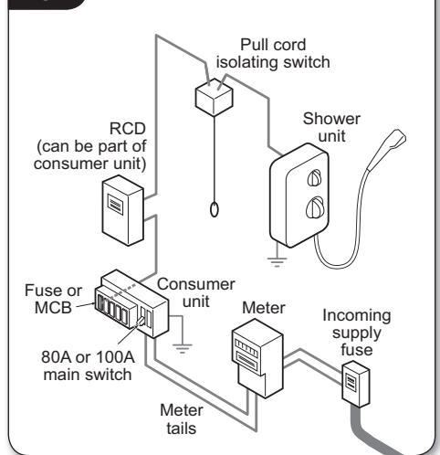
Fig.4 Schematic of installation circuit
