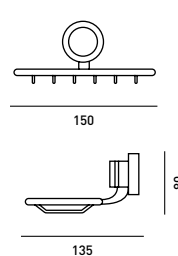
ANE014CP Wire soap basket
