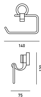
ANE001CP Toilet roll holder
