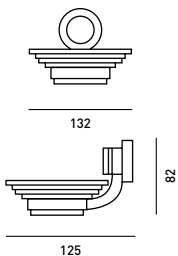
ANE004CP Glass soap dish & holder
