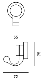
ANE009CP Robe hook
