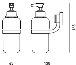
AWE015CP Liquid soap dispenser
