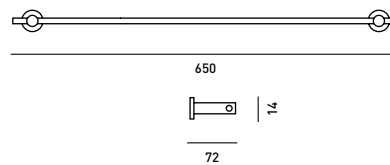
ATH246CP Single towel rail
