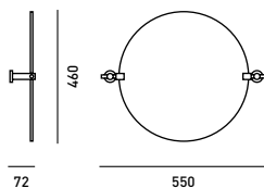
ATH013CP 18" Swivel mirror & brackets
