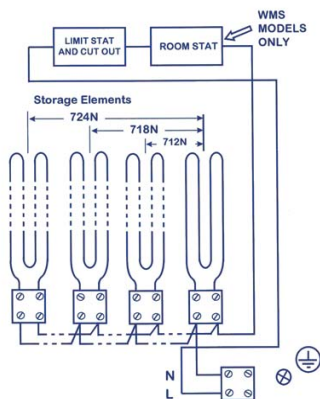
CIRCUIT DIAGRAM
