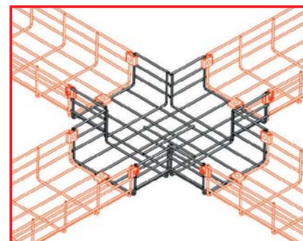
UCB-CP100x200 Connection Example
