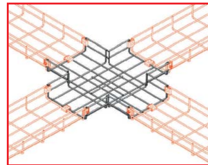
UCB-CP50x100 Connection Example
