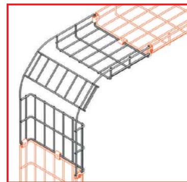
UCB-OB50x300 Connection Example
