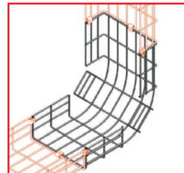
UCB-IB100x300 Connection Example
