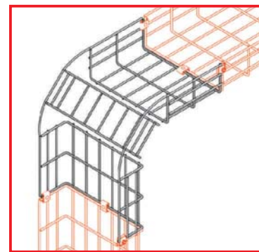
UCB-OB100x300 Connection Example
