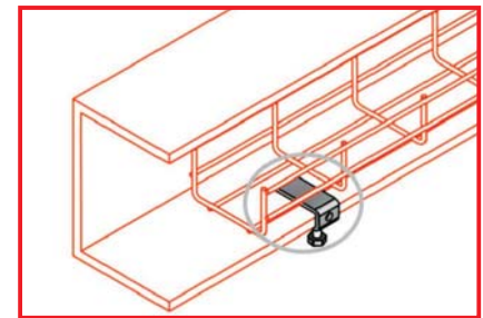
UCB-ATK-T4 Connection Example
