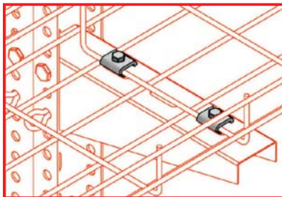
UCB-ATK-6-1-U Connection Example
