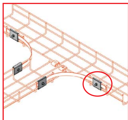
UCB-ATK-2-2 Connection Example
