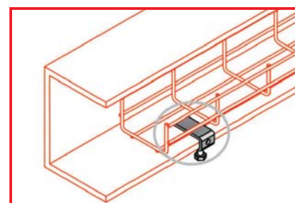
UCB-ATK-T4 Connection Example
