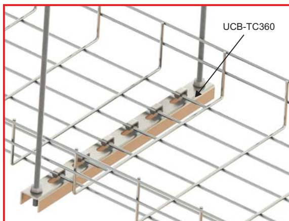
UCB-TC360 Connection Example
