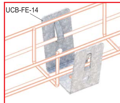
UCB-FE-14 Connection Example
