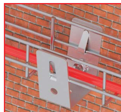
UCB-FE-14 Connection Example
