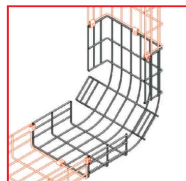
UCB-IB100x300 Connection Example
