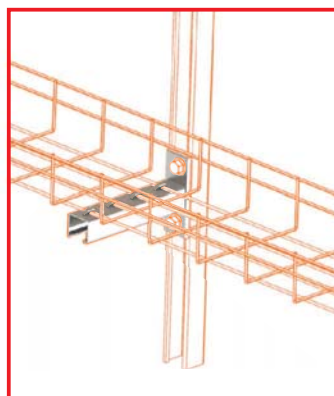
UCB-CSB-41-210 Connection Example
