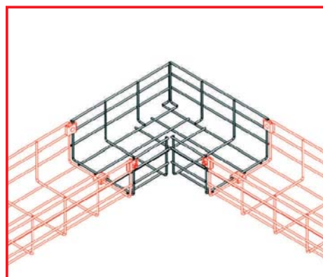
UCB-HB100x200 Connection Example
