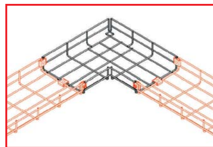
UCB-HB50x200 Connection Example
