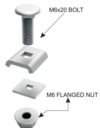
UCB-ATK-6-2 Connection Example
