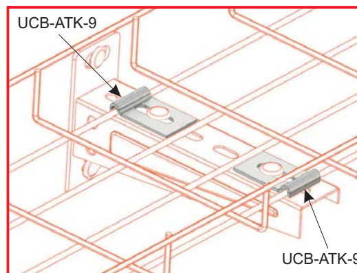
UCB-ATK-9 Connection Example
