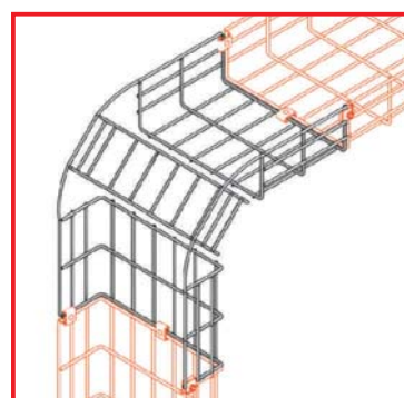
UCB-OB100x300 Connection Example
