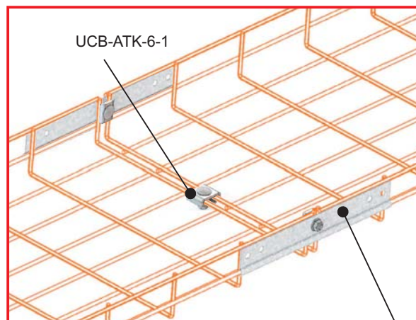
UCB-ATK-3 Connection Example UCB-ATK-3
