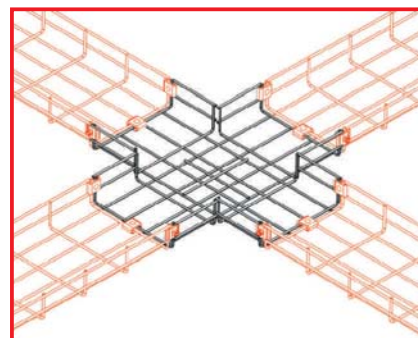
UCB-CP50x100 Connection Example
