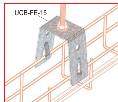
UCB-FE-15 Connection Example
