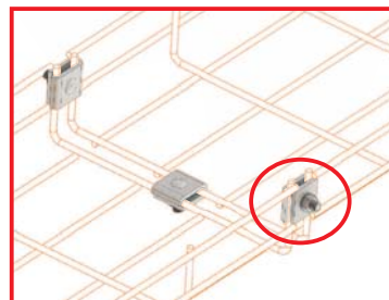
UCB-ATK-6-2 Connection Example
