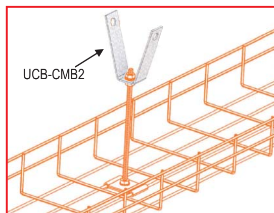
UCB-CMB2 Connection Example
