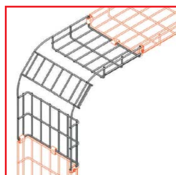
UCB-OB50x300 Connection Example
