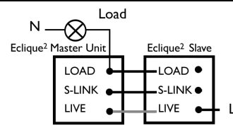
Fig 3. Alternative Wiring for Multi-Way Circuits
