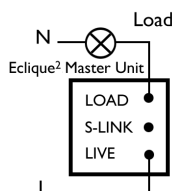
Fig 1. Wiring for 1-Way Circuits
