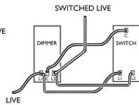
EXAMPLE WIRING 2-WAY DIMMER
