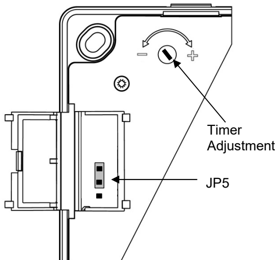
Fig.5: VASF100BF (Basic), VASF100TF (Timer)
