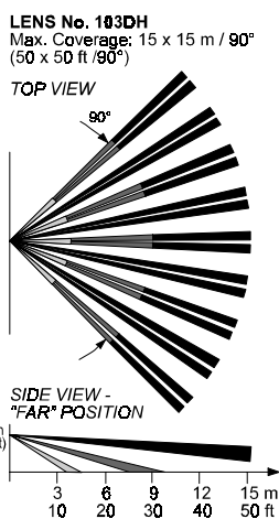
Figure 2. Coverage Pattern
