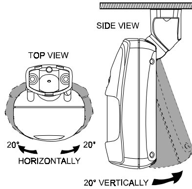
Figure 7. Tilt / Swivel Limits
