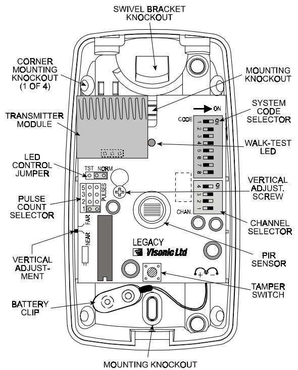
Figure 4. Inside View
