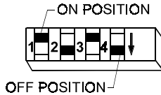
Figure 5. Channel Selector
