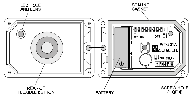
Figure 3. Inside View of the WT-201WP
