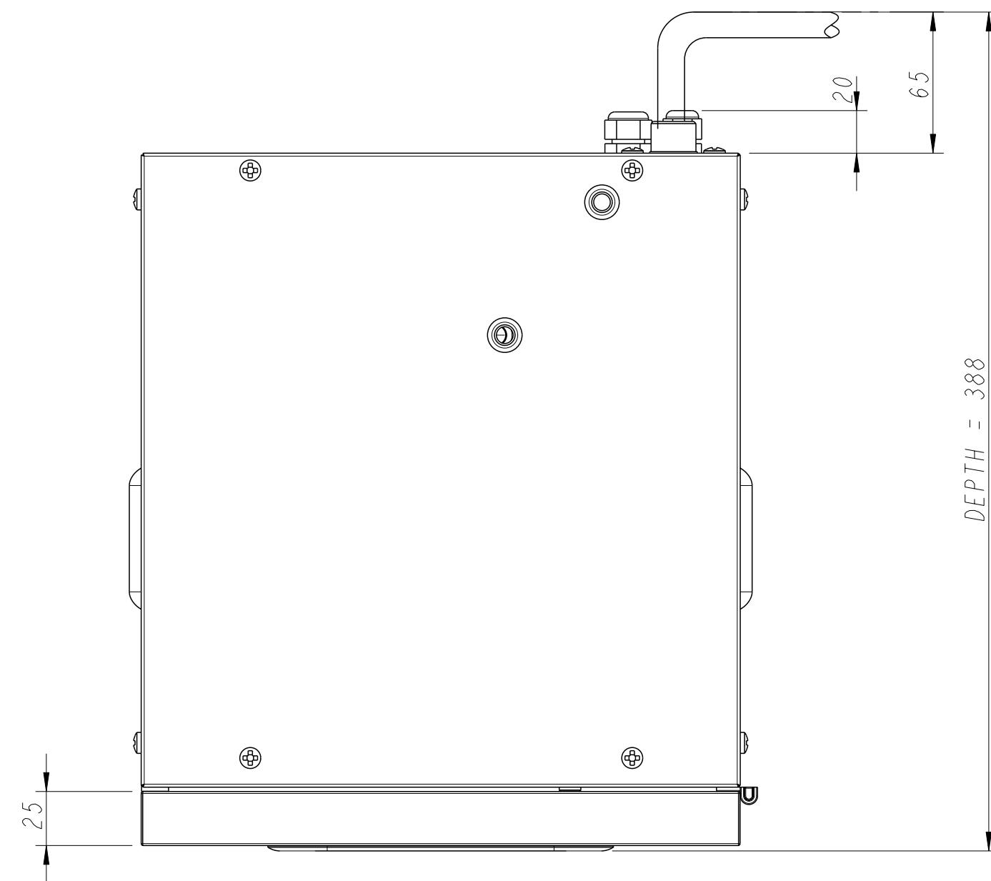
TOP VIEW
