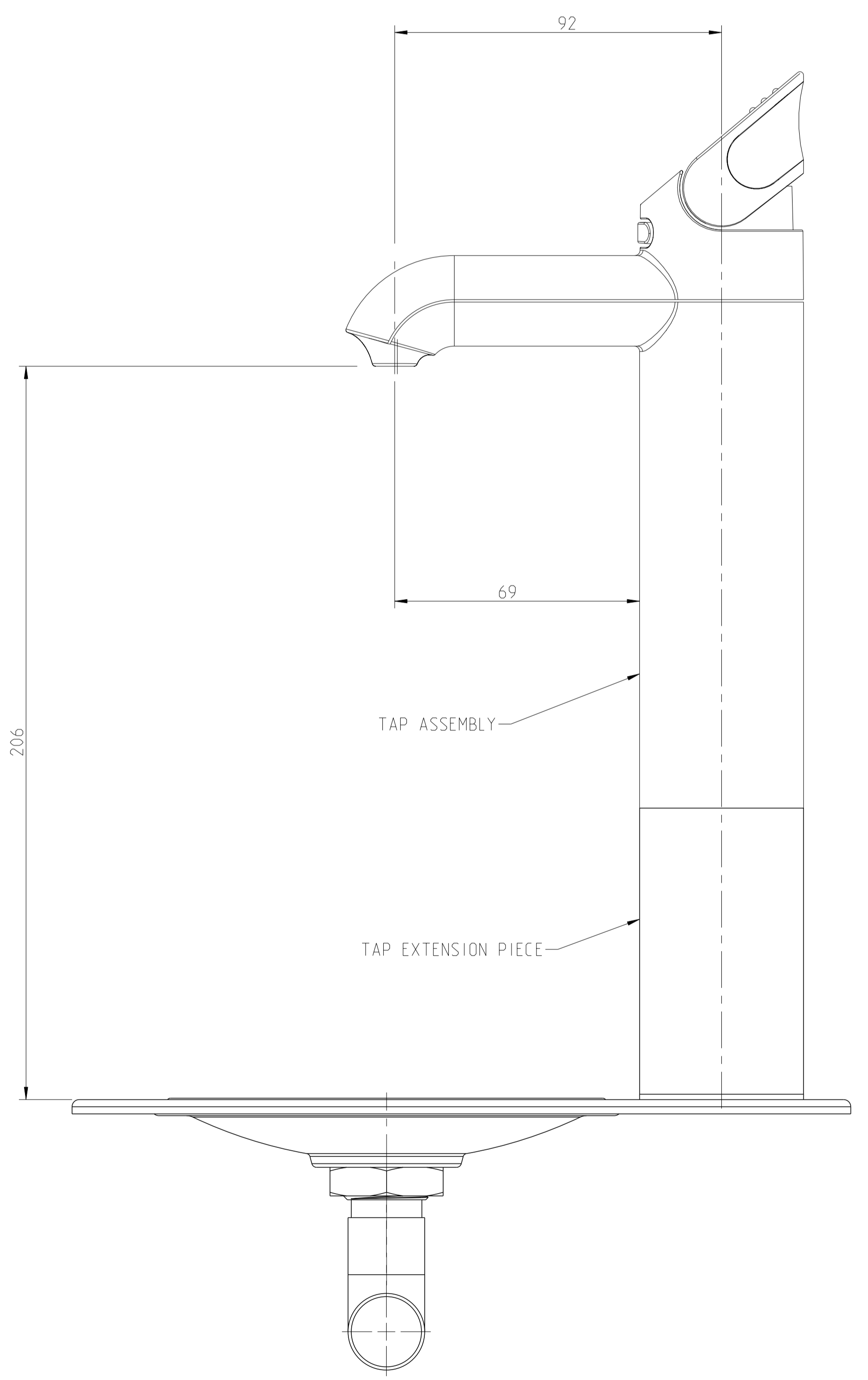
TAP ASSEMBLY MOUNTED ON FONT SCALE 1.000
