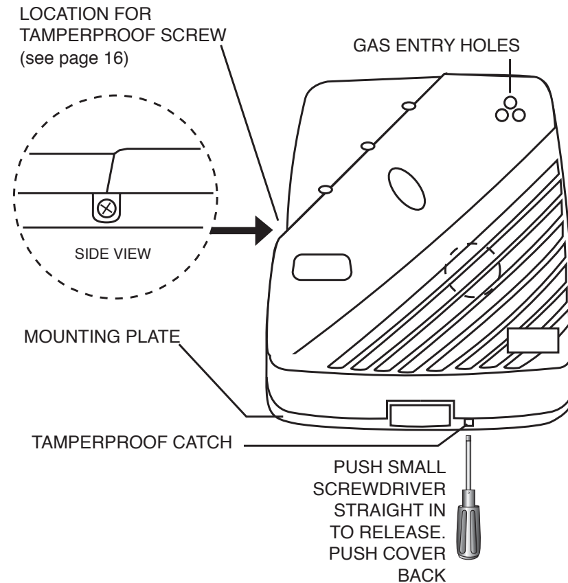
Figure 1 - Alarm Installation
