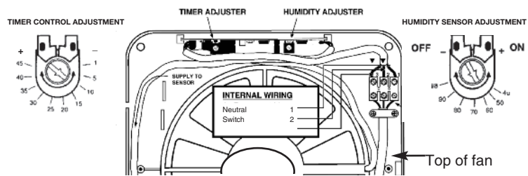
Humidity/ Timer Adjustment diagram
